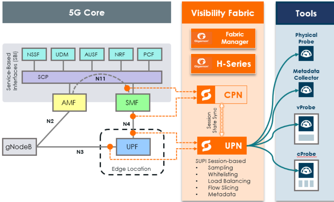
Figure 32 5G Stand Alone Packet Core Network
