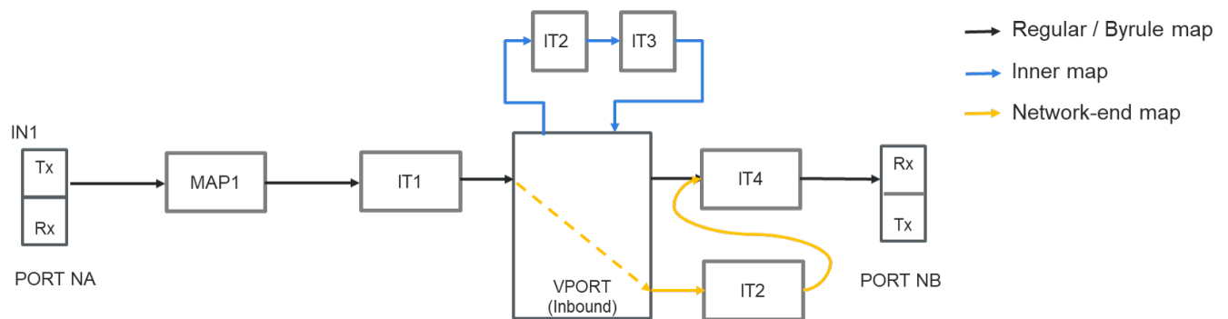
Figure 19 Flexible Inline Decryption Maps
