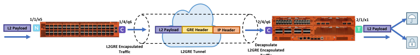
Figure 30 L2GRE Tunnel Encapsulation and Decapsulation
