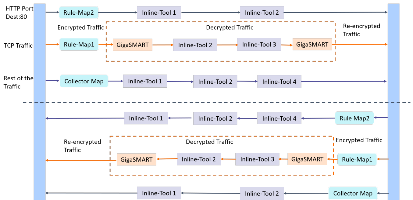
Figure 18 Flexible Inline Decryption Solution
