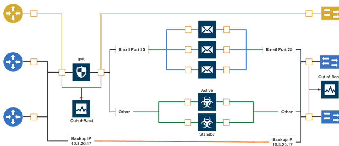
Figure 15 Flexible Inline Arrangements Scenario
